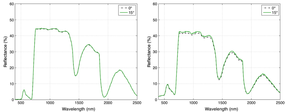
Fig. 10 Subsurface reflectance curves computed for specimens (a) S1 and (b) M1 considering two angles of incidence. The curves were obtained using the ABM-B and ABM-U models 15 and the data provided in Table 1.
